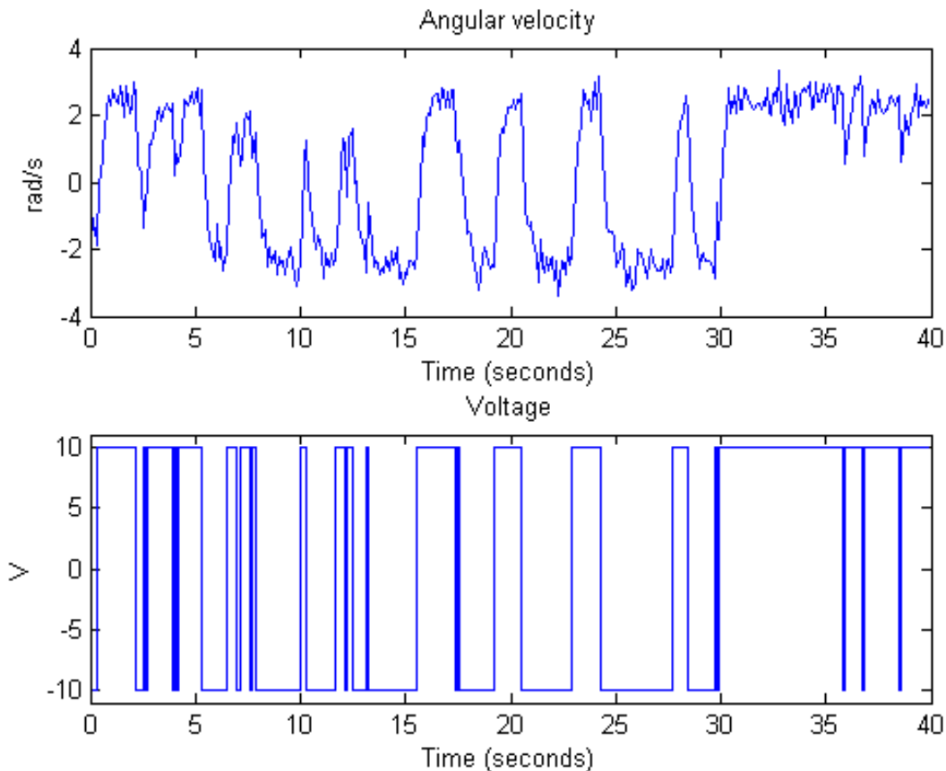
Figure 2: Input-output data from a DC-motor.
