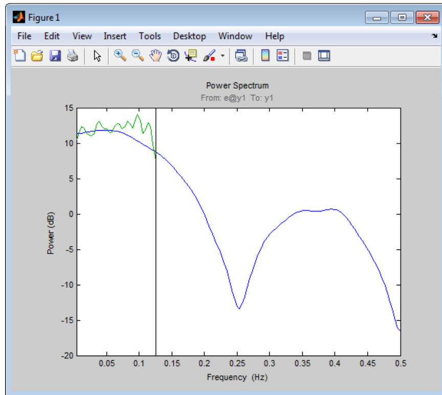
Folding Effects with Manual Decimation
