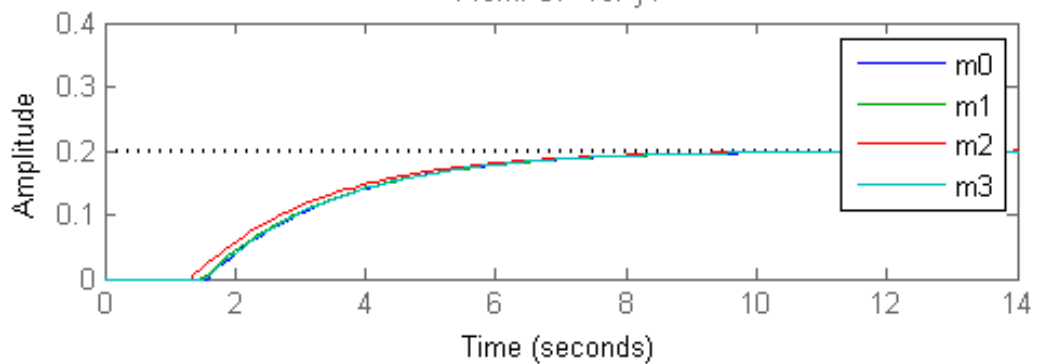
Step Response From: u1 To: y1
