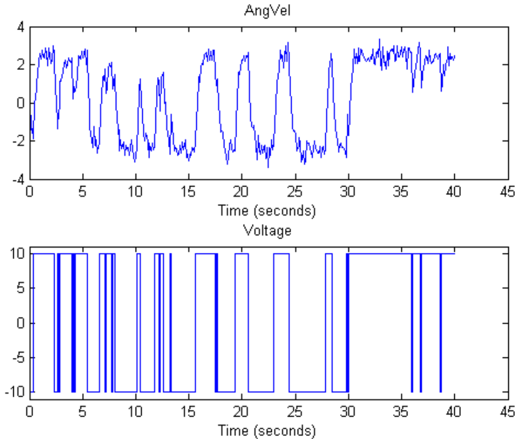
Figure: Measurement Data: Voltage to Angle
